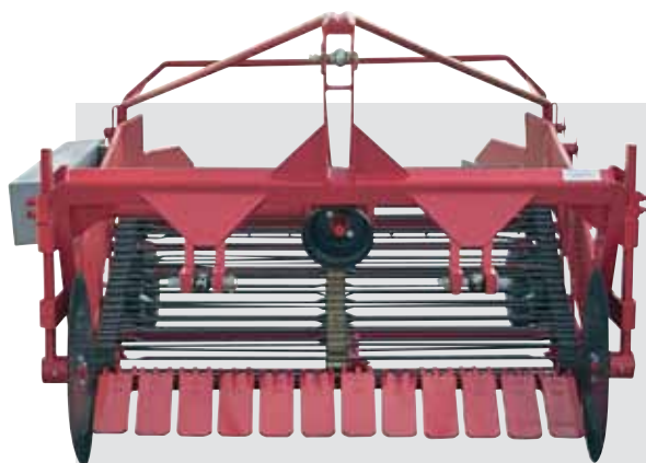
Πατατοεξαγωγέας SPE Extractor-Potato machine SPE
